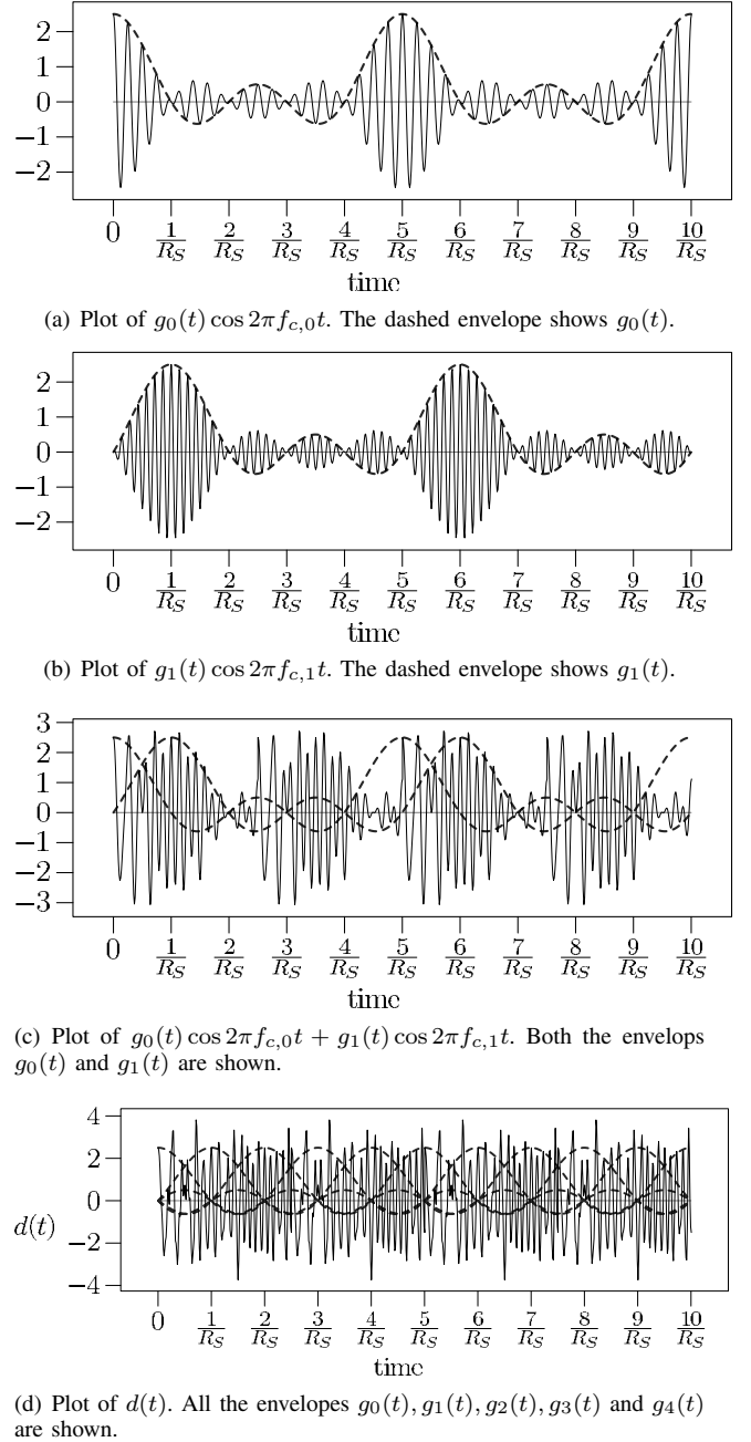
Fig. 2. Down-conversion function.
