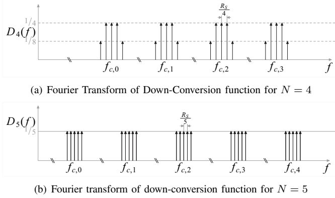
Fig. 3. Fourier transforms of down-conversion function for N = 4 and N = 5 .
